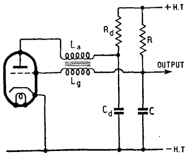
Fig. 1. The usual blocking-oscillator saw-tooth generator.
