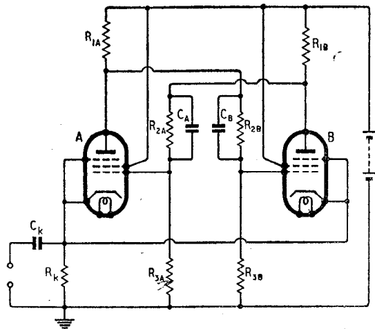
Fig. 1. Scale of two counter circuit.
