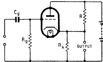
Fig. 3. Cathode-follower buffer circuit.
