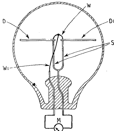
Thermocouple for centimetre field-strength measurement.
