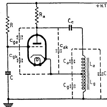
Fig. 6. Cathode-tapped blocking-oscillator circuit.
