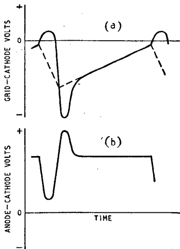
Fig. 3. Grid (a) and anode (b) voltage waveforms with heavy transformer losses. The dotted curve shows the voltage across C.
