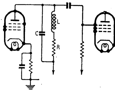
Fig. 2. Skeleton circuit of i.f. amplifier stage.
