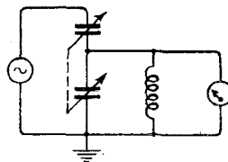
Fig. 2. Injecting r.f. through a ganged feeder capacitor.
