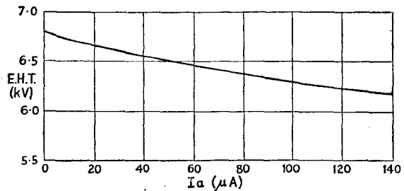
REGULATION CURVE OF E.H.T. SUPPLY
