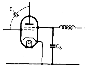
Fig. 5. Before a screened-grid stage can be assumed free from liability to oscillate through back-coupling, attention should be paid to external stray capacitance ( C_1 ), and the inductance of the wiring drawn in heavy line.
