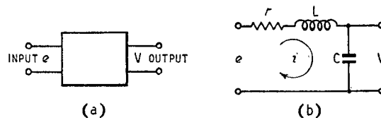
Fig. 1. Circuit magnification.
