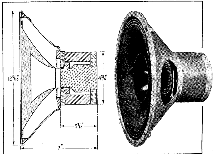
Goodmans "Axiom 22" loudspeaker. The sectional drawing shows the general arrangement of the ring magnet and polepieces.
