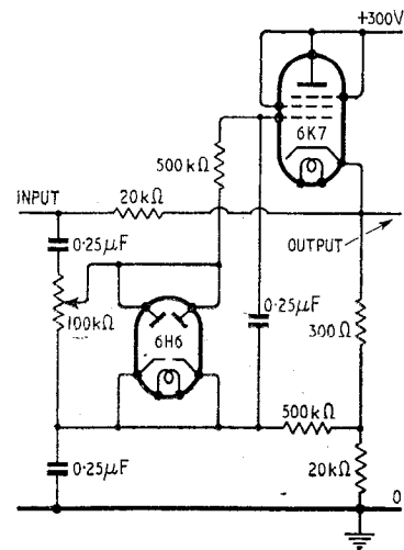
Fig. 3. Cathode-follower contrast expander.
