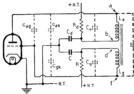
Fig. 5. Blocking oscillator circuit with the stray capacitances added.
