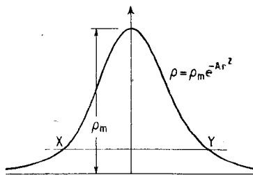
Fig. 2. This Gaussian curve shows the electron density \rho in a cross-section of the beam at the crossover.
