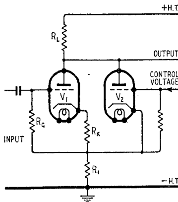
Fig. 4. Contrast expansion by negative feedback. V_2 and R_1 constitute the control potential divider.
